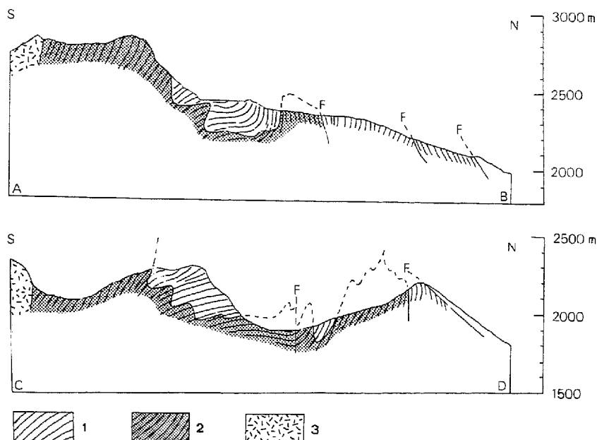
Fig. 3. Cross sections through the studied area showing main phase cleavage and folding of the lower conglomerate boundary. Both folding and cleavage are of Variscan age. Legend: 1 = Upper Ordovician; 2 = pre-Upper Ordovician; 3 = porphyritic biotite granite. See figure 2 for location of sections.
