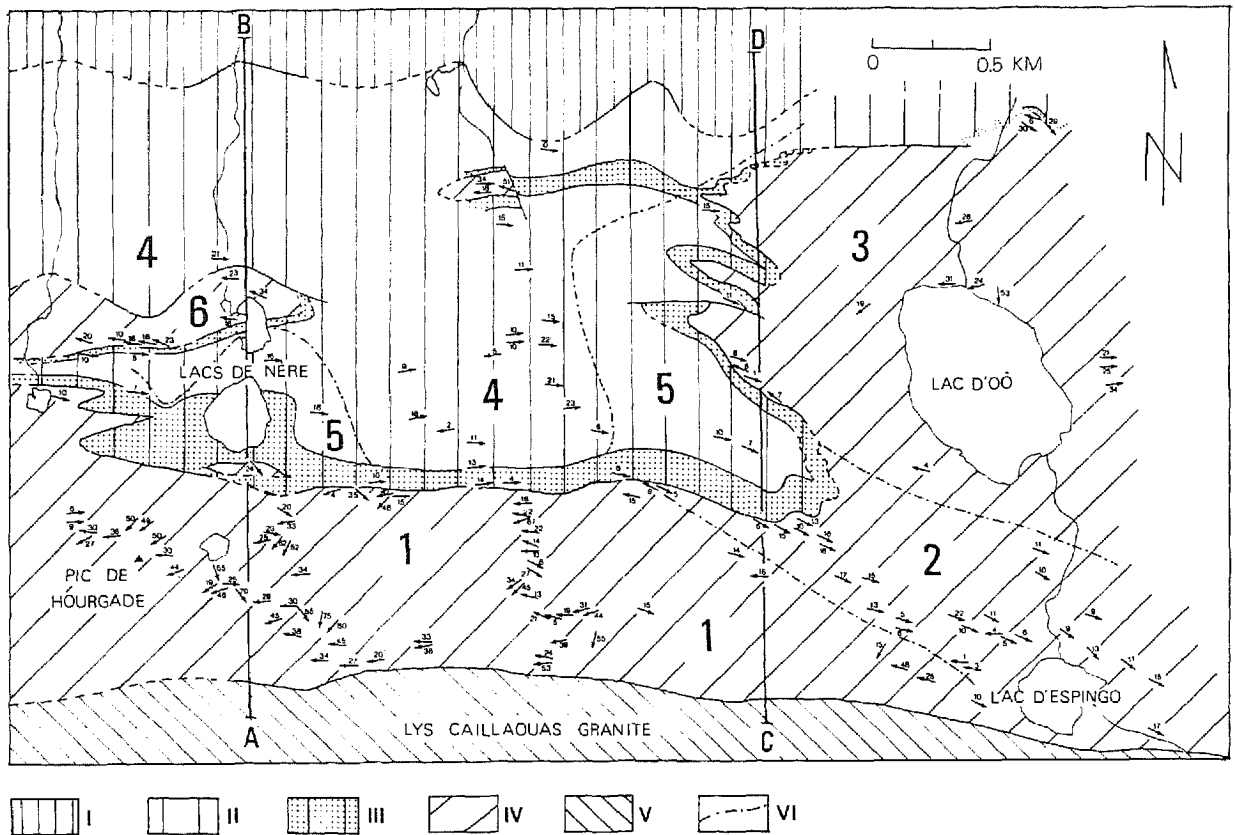
Fig. 2. Simplified geological map of the studied area showing \delta -lineations within the Cambro-Ordovician rocks of the central Lys-Caillaouas area. Each arrow indicates one measurement. Numbers indicate plunge. Large numbers, 1 to 6, mark sub areas with relatively constant orientation of main phase cleavage and/or \delta -lineations. Legend: I = Silurian & Devonian; II = Upper Ordovician mica schists and quartzitic marbles; III = Upper Ordovician conglomerate; IV = pre-Upper Ordovician mica schists, quartzites and quartzitic marbles; V = porphyritic biotite granite; VI = boundary between subareas with relative constant orientation of \delta -lineations and/or main phase cleavage (see Fig. 4).
