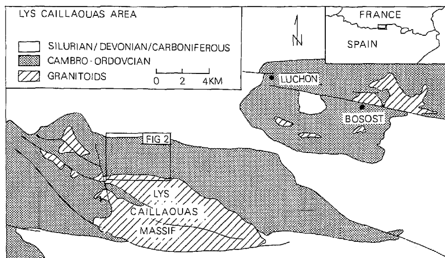
Fig. 1. Geological sketch-map of Lys Caillaouas area (after Zwart 1979) showing location of the studied area.
