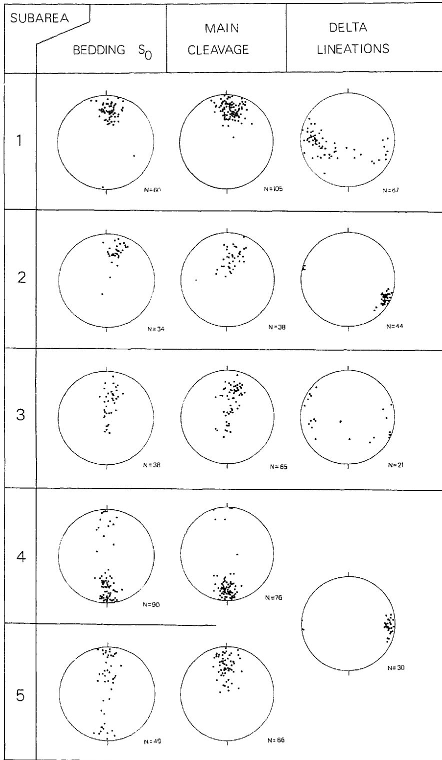
Fig. 4. Stereographic equal area projections per subarea showing poles on sedimentary bedding, poles on main phase cleavage and \delta -lineations. Subareas are indicated in Fig. 2.
